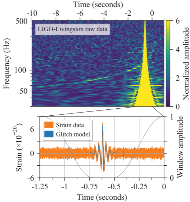
Figure 10: Demonstration of the glitch model template (blue) and the glitch (orange) overlapping one another to cancel out the noise. Credits: LIGO
