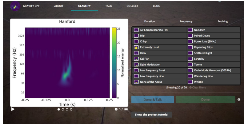
Figure 5: Gravity spy - citizen science project that helps classify glitches detected by LIGO's interferometers. Credits: Zooniverse, Gravity Spy.
