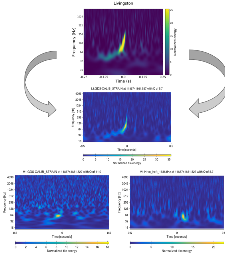
Figure 8: Demonstration of a signals from Gravity Spy (top) in relation to the Livingston Spectrogram signal (middle). Handddford (bottom left) experienced a very faint signal, same as Virgo (bottom right). But all observatories experienced the same detection.
