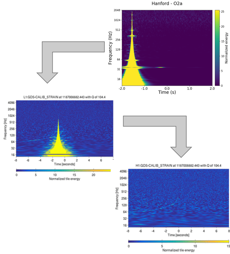
Figure 9: Binary neutron star from Livingston with glitch overlying the detection (middle). The glitch from Livingston template matched with a Gravity Spy signal (top). Handford (bottom) showed a clean gravitational wave signal.
