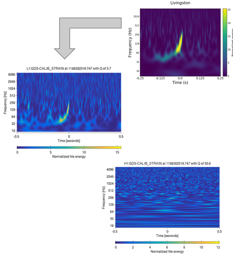
Figure 7: Demonstration of a signals from Gravity Spy (top right) in relation to the Livingston Spectrogram signal (middle). Handford (bottom) experienced a very faint signal, impossible to see with the human eye unless quality and parameters are changed.
