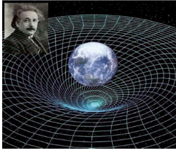
Figure 1: Massive objects bending spacetime. Credits: NASA.
