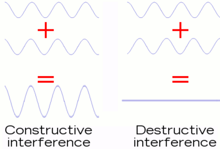
Figure 4: Interference patterns when two waves merge. Credits: LIGO CalTech.
